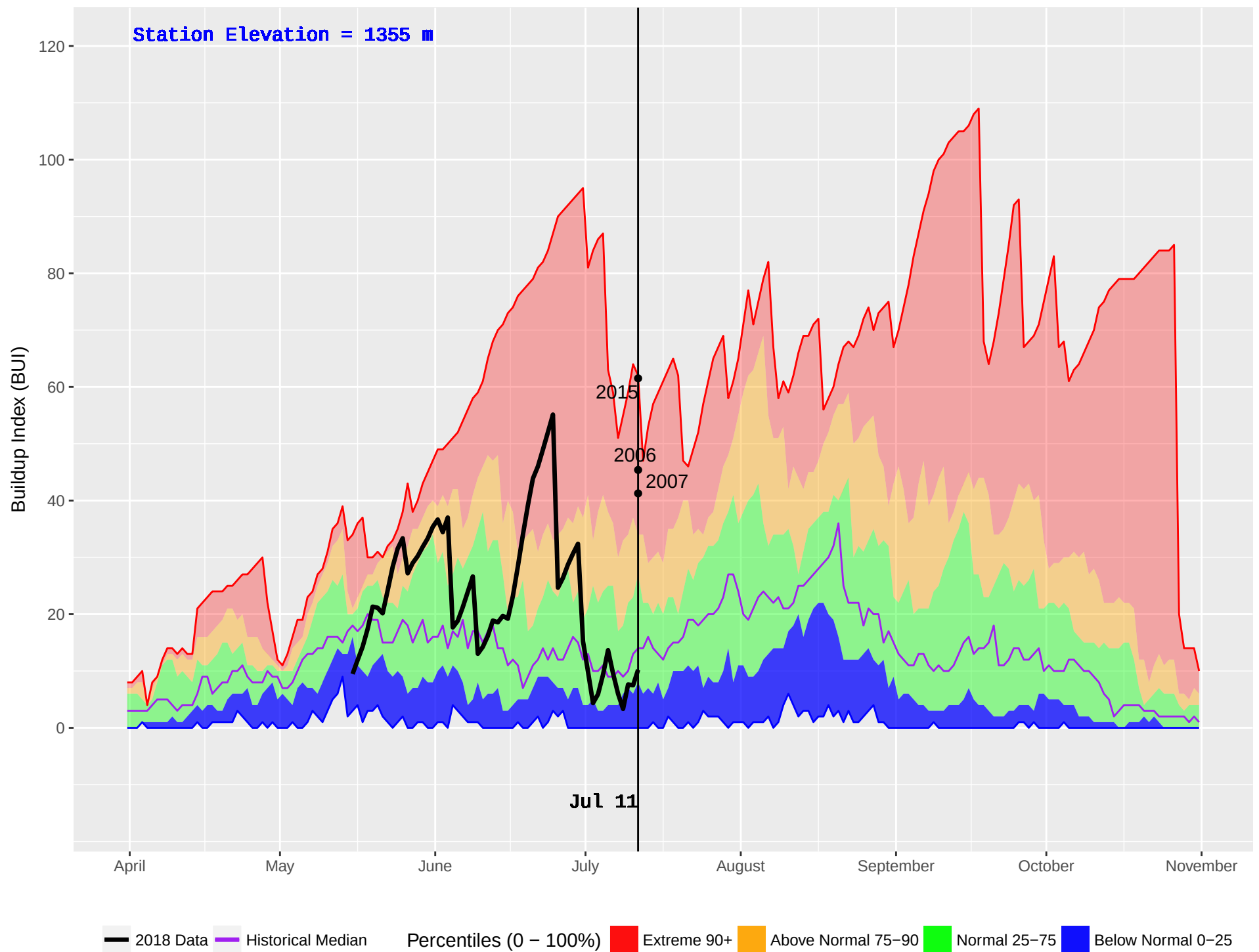
BIG VALLEY (262) : Historical (1987–2016) and Current (2018) Noon Buildup Index (BUI)
