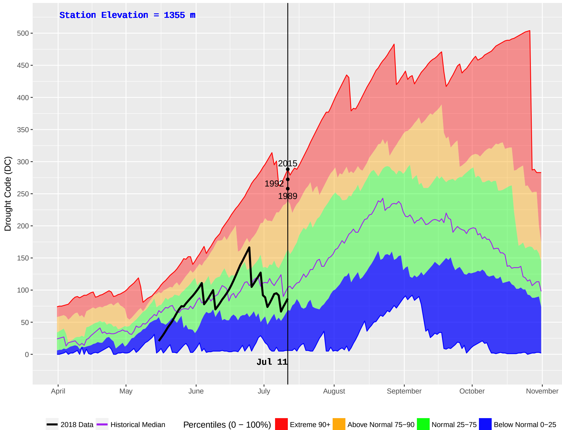
BIG VALLEY (262) : Historical (1987–2016) and Current (2018) Noon Drought Code (DC)
