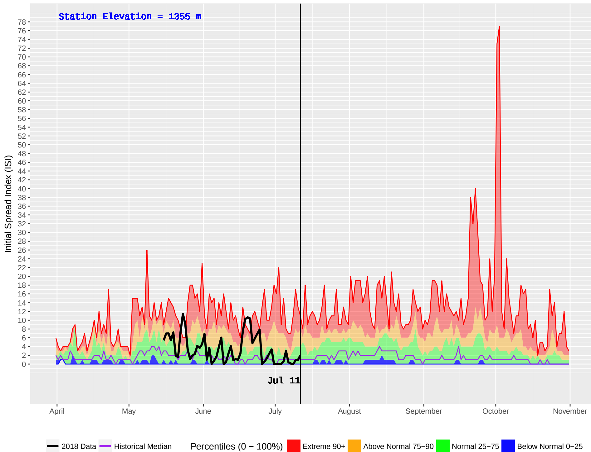
BIG VALLEY (262) : Historical (1987–2016) and Current (2018) Noon Initial Spread Index (ISI)
