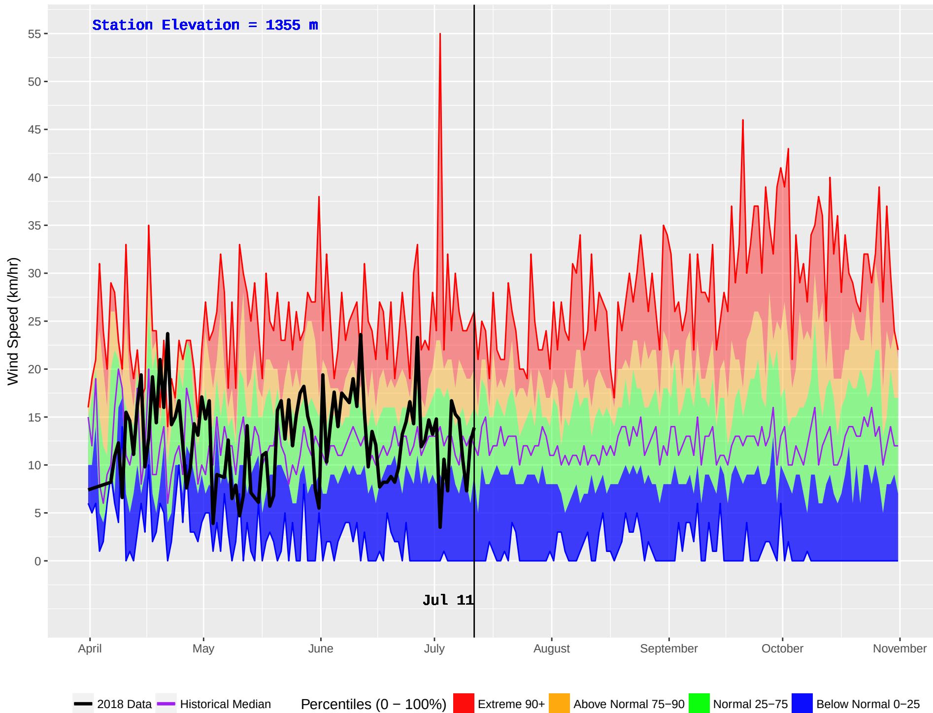
BIG VALLEY (262) : Historical (1987–2016) and Current (2018) Noon Wind Speed
