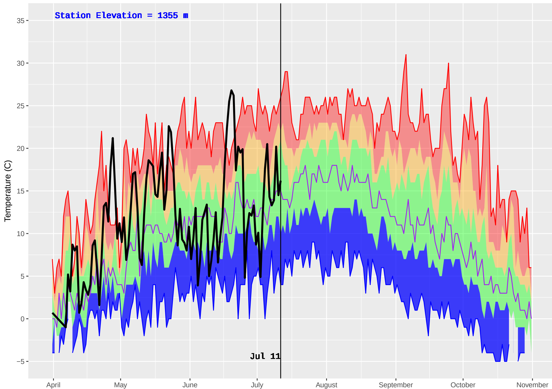
BIG VALLEY (262) : Historical (1987–2016) and Current (2018) Noon Temperature
